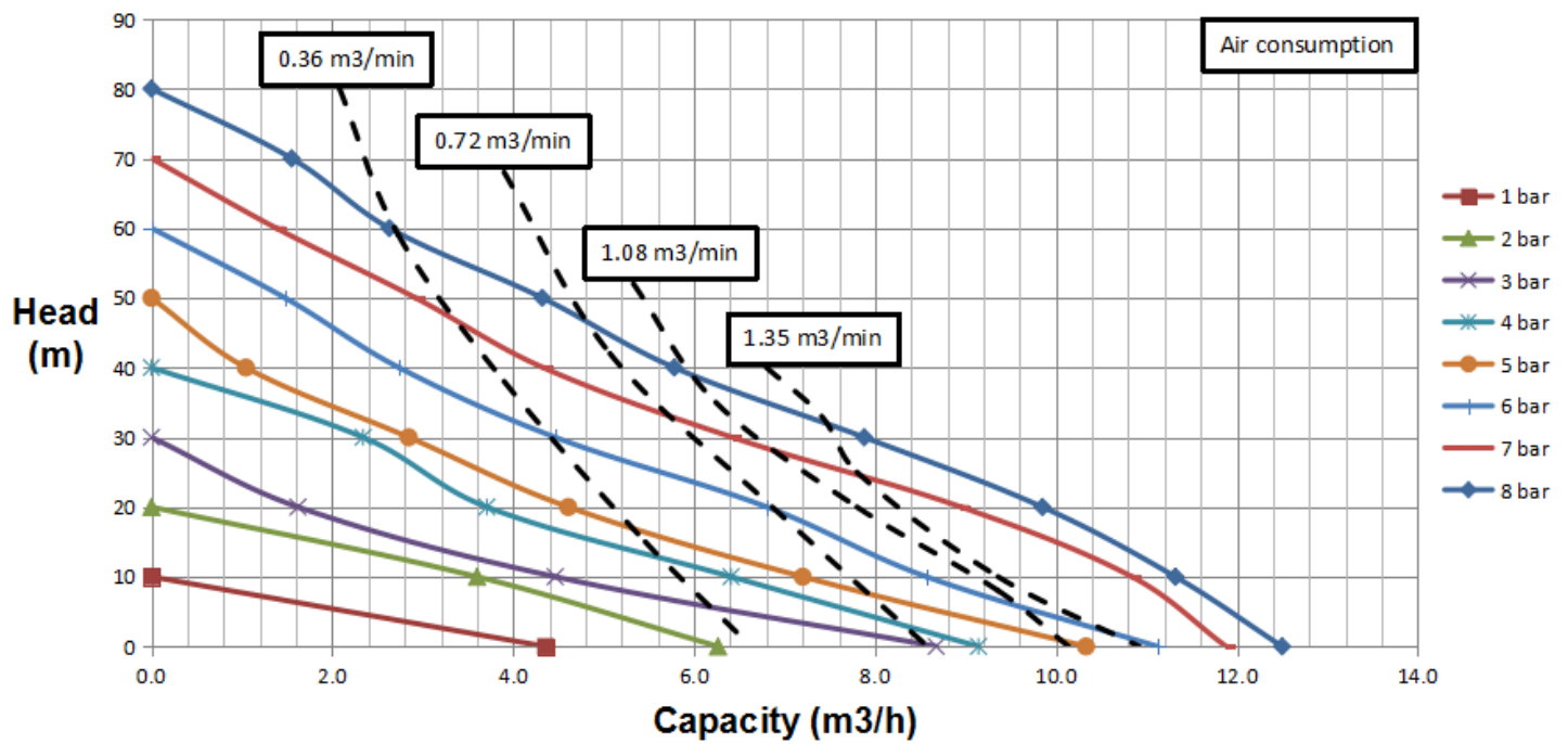
TDPKN-40 pump performance curve
