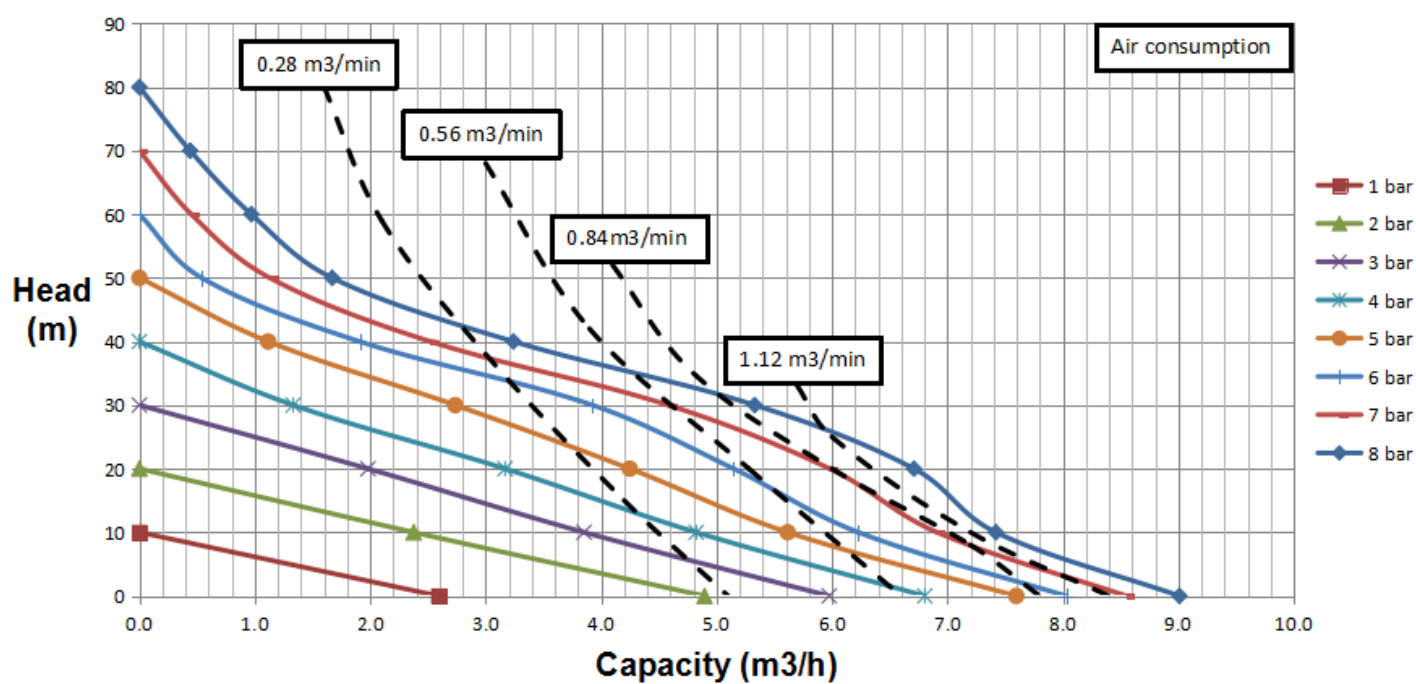
TDPKN-25 pump performance curve
