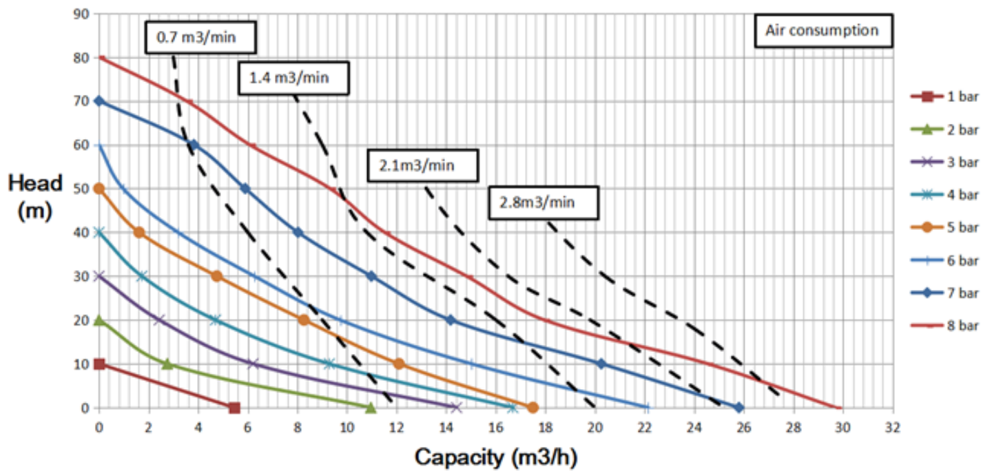
TDPK-50 pump performance curve
